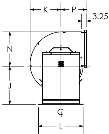
DRIVE SIDE VIEW
